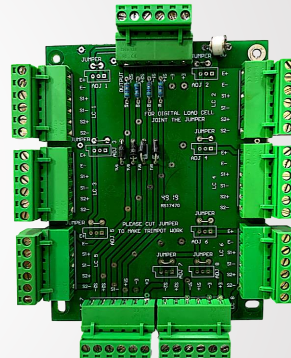
JB-8 (8 DIGITAL LOADCELLS)
