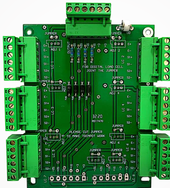
JB-6 (6 DIGITAL LOADCELLS)
