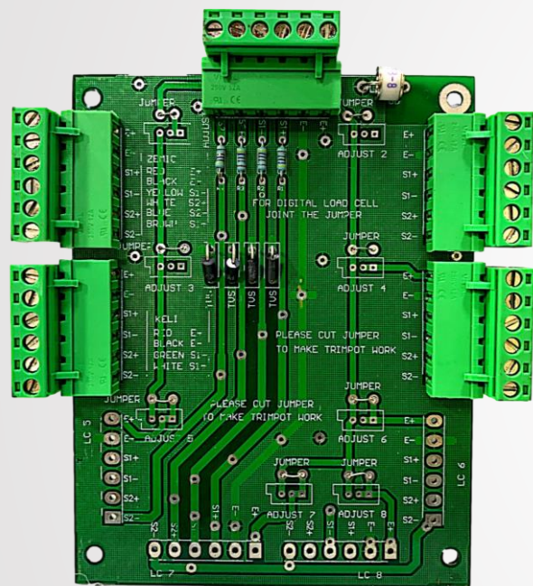
JB-4 (4 DIGITAL LOADCELLS)
